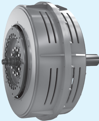
KFBD - FLUID COUPLING PTO For internal combustion engines, up to 500 kW
