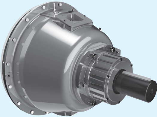
HF SERIES - OIL OPERATED POWER TAKE OFF Up to 800 kW
