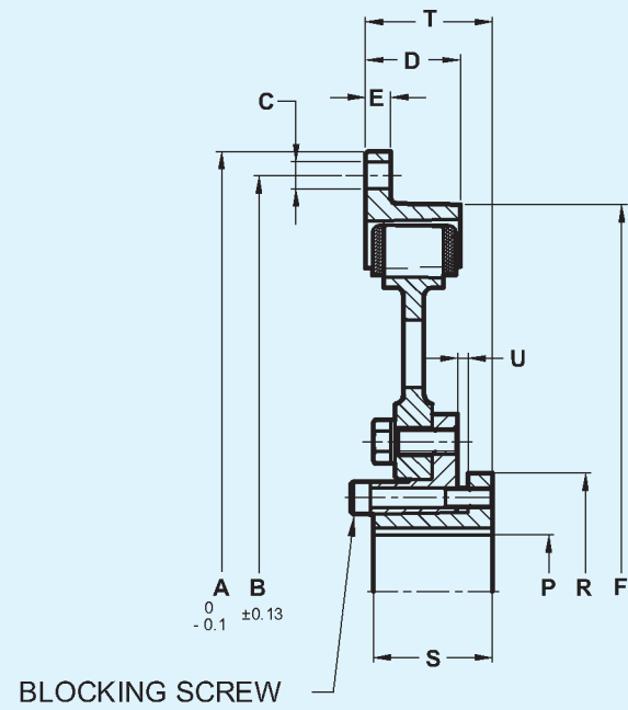
RBD-QD WITH SINGLE RUBBER BLOCKS
