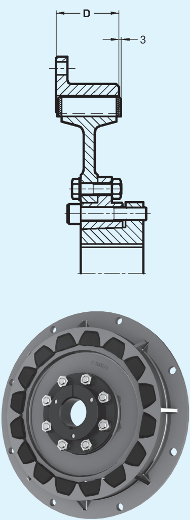
RBD-QD WITH DOUBLE RUBBER BLOCKS
