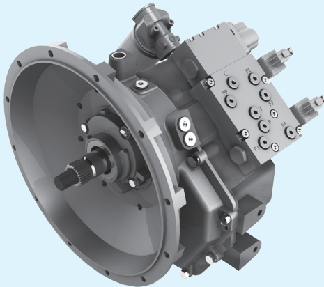
POWER SHIFT TRANSMISSION Electric selector, up to 95 kW
