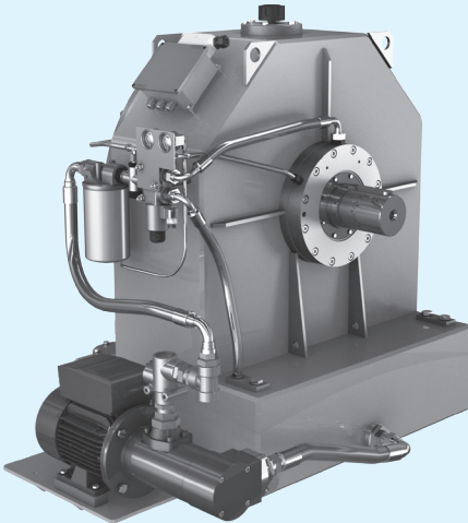
SH-SHC - HYDRAULIC CLUTCH Up to 2500 Nm
